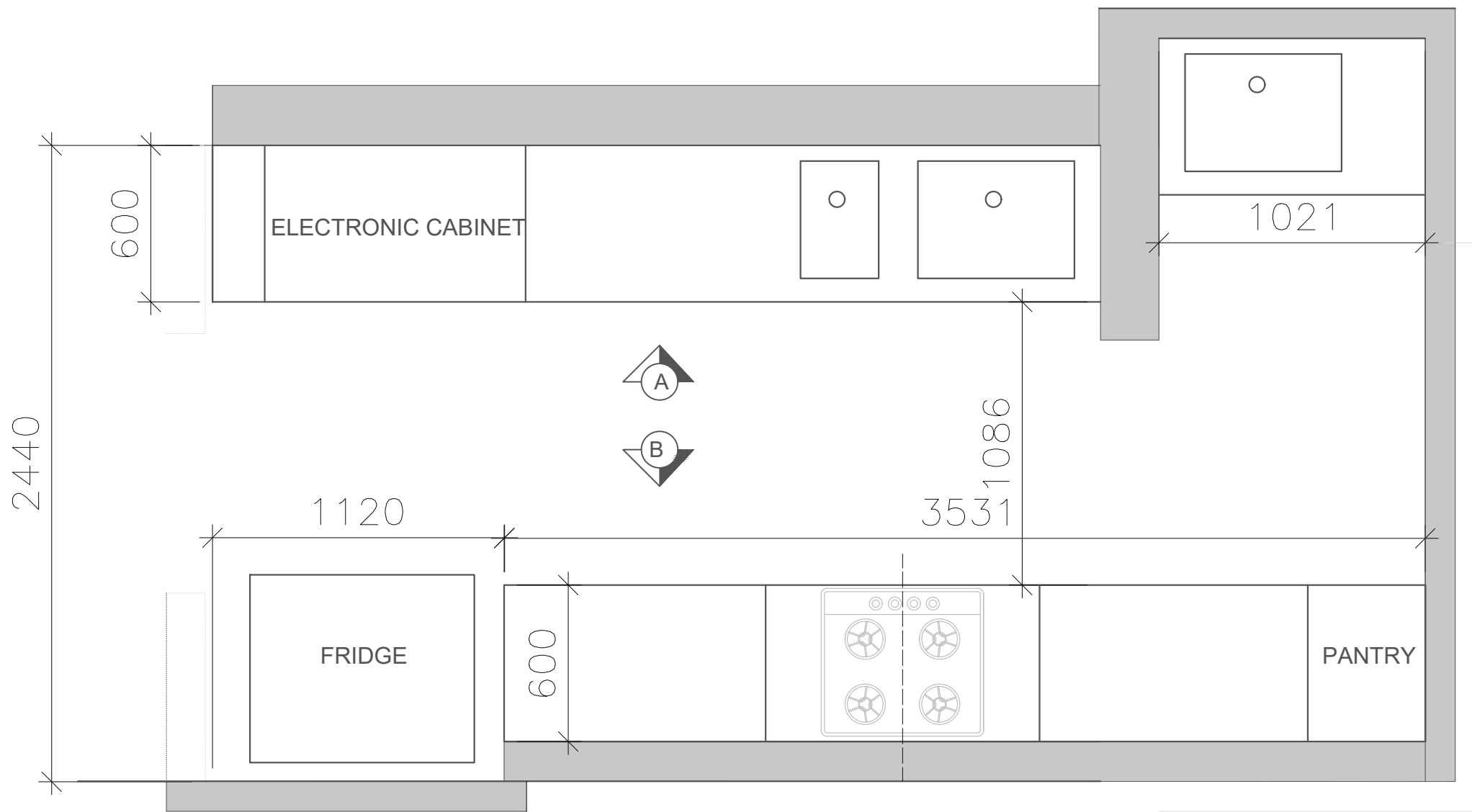
PLAN
